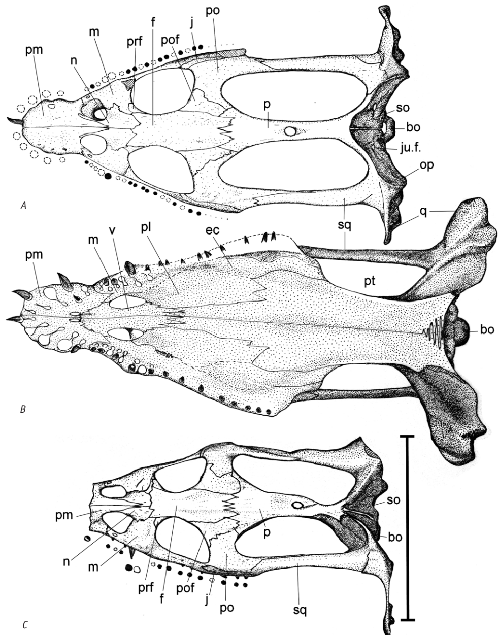
Fig. 1. Three skulls of Nothosaurus marchicus . A – TW480000375 in dorsal view; B – TW480000376 in ventral view; C – TW480000378 in dorsal view. bo, basisoccipital; eo, exoccipital; ec, ectopterygoid; f, frontal; j, jugal; ju.f., jugular foramen; m, maxilla; n, nasal; op, opisthotic; p, parietal; pmx, premaxilla; po, postorbital; pof, postfrontal; prf, prefrontal; pt, pterygoid; q, quadrate; sq, squamosal. Filled in circles next to the skull represent tooth elements visible in lateral view, open circles represent assumed tooth positions. Scale bar represents 5 cm.
