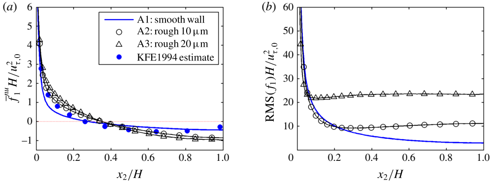
FIGURE 5. (Colour online) Non-uniform part (a) and RMS (b) of the particle drag force in the streamwise component of the gas momentum equation, \bar{f}_1^{nu} and RMS(f_1) , normalized with \rho u_{\tau,0}^2/H . Laden simulations A1 (solid, no markers), A2 (solid, circles) and A3 (solid, triangles). In (a) an estimate based on experimental results (KFE1994) is also shown, as described in the text.
