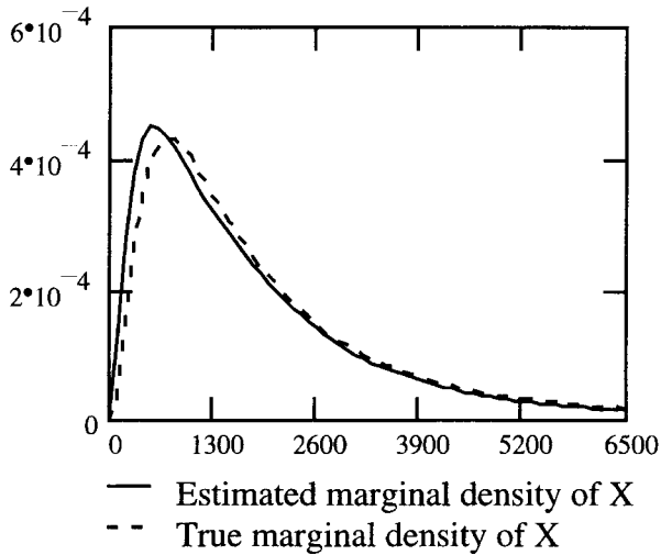
FIGURE 4.2: Estimated and True Marginal Densities of Claims.
