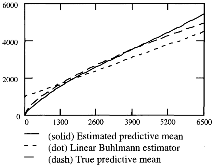
FIGURE 4.3: Credibility Estimators.
