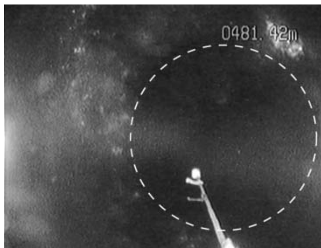
Fig. 14. Indistinct exit cavity in the 'honeycomb' ice at the borehole base, as captured by the down-looking camera.
