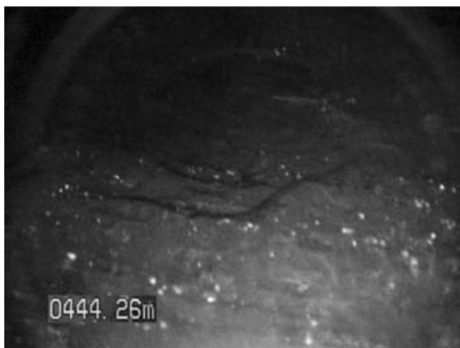
Fig. 12. Large borehole wall cavity (upper half of image) in the marine ice layer at depth. The ledge in the lower half of the image has neither settled nor entrained debris evident here.
