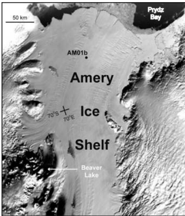
Fig. 1. Map of northern half of the AIS, and AM01b borehole location. Local snowfall accumulates over this part of the shelf ( 300 \text{ kg m}^{-2} \text{ a}^{-1} at the drill site). Further south the shelf passes through a superimposed- and bare-ice ablation zone with continental ice exposed at the surface.
