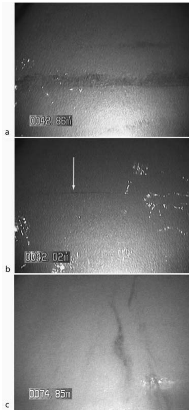
Fig. 3. (a) Thick 10–15 mm refrozen summer meltwater ice lens still preserved after the firn has compacted to bubbly glacial ice. (b) Thin (1–2 mm) wind-glazed crust ice lens (arrowed) preserved in granular bubbly glacial ice. (c) Vertical refrozen (2–10 mm thick) meltwater ice veins near the top of the continental ice layer. Note: all side-looking frames in this paper have had the image digitally inverted so that the top of the image is up in the ice. In the original recording by the probe, up in the image was down in the ice (Carsey and others, 2002).
