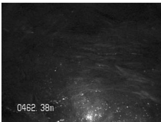
Fig. 13. The flaky layered texture of the marine ice (difficult to capture in still frames) showing a structural network rather than an aggregation of loose slush near the ice-shelf base.
