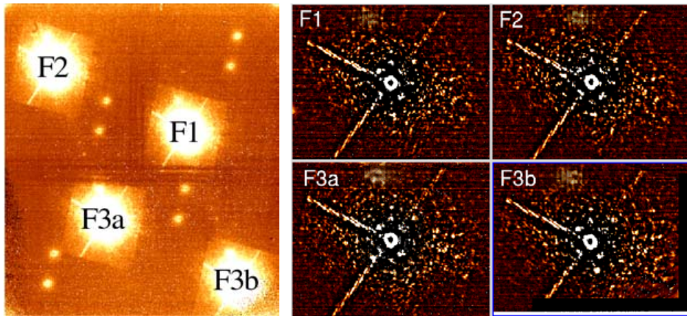
Figure 1. Left: Two minutes of raw SDI data from NACO SDI's 1024 \times 1024 Aladdin array in the CONICA AO camera (Lenzen et al. 2004). Right: Same dataset, slightly processed. Apertures have been selected around each filter image. In order to reveal the speckle pattern, a heavily smoothed image was subtracted from the raw images (unsharp masking). The resulting speckle patterns are very similar between the 4 simultaneous images which means that an effective subtraction of speckles can be obtained between the filters.
