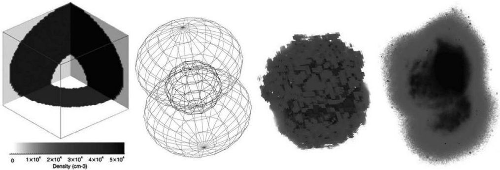
Figure 1. (Left) Density distribution, cross section, and morphology used for NGC 7027. (Right) Computed surface brightness in the He II \lambda 4686 line compared with the HST image.
