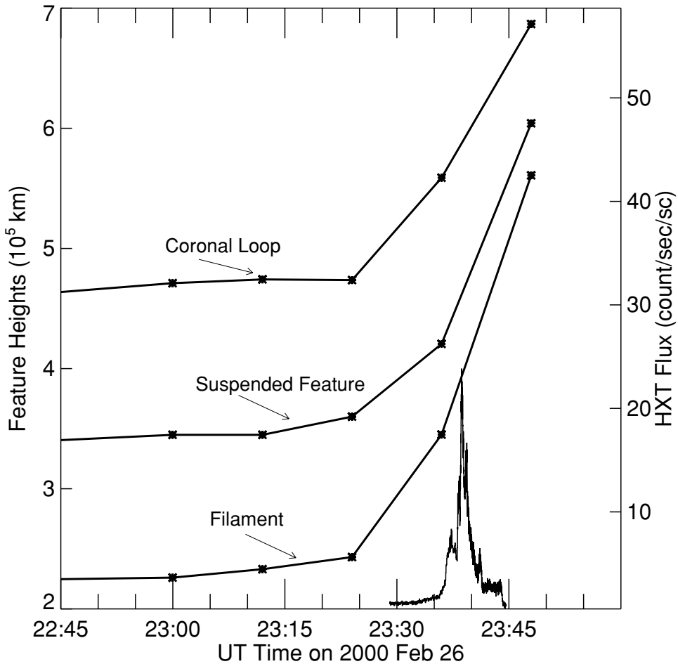
Figure 3. Trajectories of the filament, suspended feature, and coronal loop as functions of time for the eruption of 2000 February 26 (Event 3), measured projected against the disk in EIT images; flux from the Lo channel of Yohkoh 's hard X-ray telescope (HXT) is overplotted from 23:29 UT. Slow pre-eruption motion starts near 23:00 UT and fast eruption starts near 23:25 UT.
