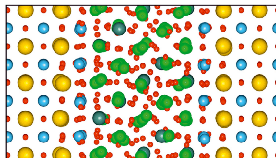
Fig. 2. (Color online) Structure of the 1 nm YSZ layer sandwiched between layers of STO at 360 K as determined by DFT MD calculations viewed down the \langle 100 \rangle STO axis. Sr atoms are shown in yellow, Ti in blue, Zr in green, Y in gray, and O in red. The YSZ O sublattice disorder is comparable to that seen at 2000 K in the strained bulk. Reproduced from [16].
