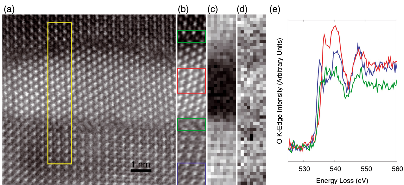
Fig. 14. (Color online) (a) High resolution ADF image of an incoherent island of YSZ surrounded by STO. (b) ADF image recorded simultaneously with a SI recorded in the area indicated by the yellow box in (a). Ti and O elemental maps extracted from the SI are shown in (c) and (d) at the same scale as (b). The O K-edge extracted from the regions indicated by the corresponding colors in (b) are shown in (e). The green spectrum shows a significant reduction in the continuum region of the spectrum, indicating the presence of O vacancies.
