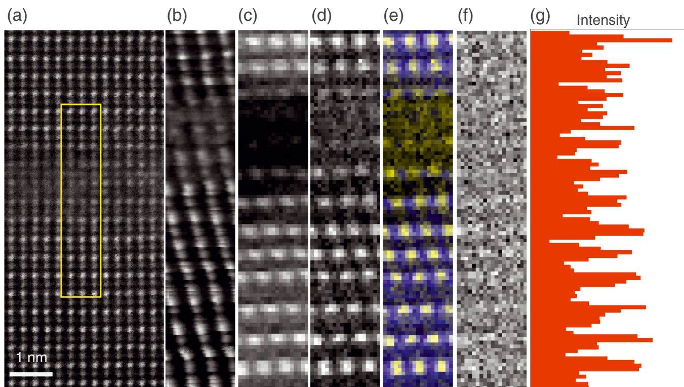
Fig. 12. (Color online) (a) High resolution ADF image of a section of coherent YSZ/STO multilayers viewed down the \langle 110 \rangle STO axis. An ADF image recorded simultaneously with a SI taken in the area indicated by the yellow box is shown in (b). Integrated Ti L and O K-edge intensity elemental maps extracted from the PCA processed SI are shown in (c) and (d) and as a composite map in (e) in which O intensity is shown in yellow and Ti intensity is shown in blue. An O elemental map extracted from the SI without PCA processing is shown in (f), and the integrated intensity of each row of pixels in the raw O map is shown in (g). The intensity is given in arbitrary units, with the background subtracted to improve the contrast.
