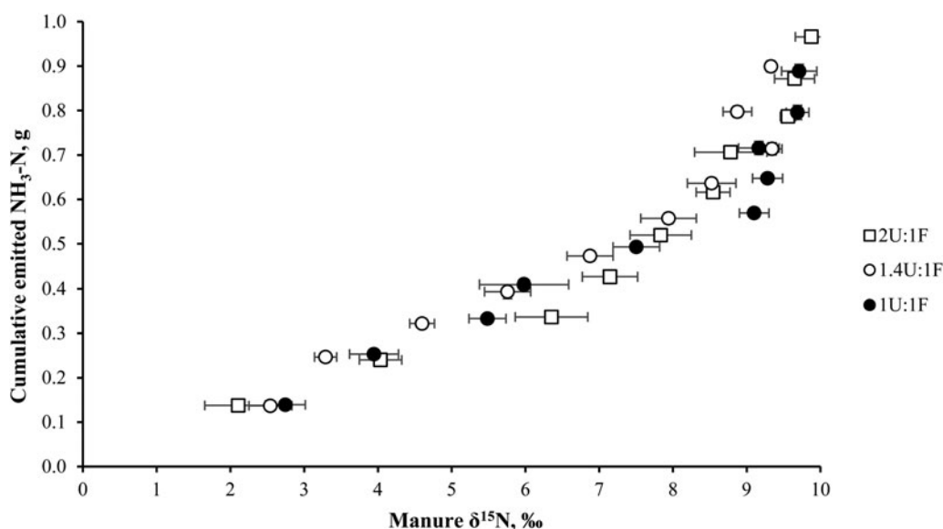
Figure 3. Relationship between cumulative emitted ammonia-nitrogen (NH 3 -N) from manure and manure N isotopic discrimination ( \delta^{15}\text{N} ) during Experiment 2: 2U:1F, ratio of urine to faeces = 2:1; 1.4U:1F, ratio of urine to faeces = 1.4:1; 1U:1F, ratio of urine to faeces = 1:1. The error bars show standard error (S.E.).
