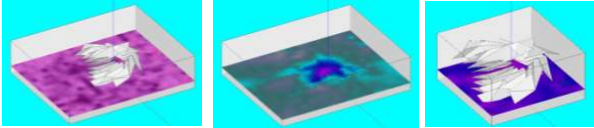
Figure 8. Axonometric view of spatial mappings of T20 with a visible Phoenix (left) and C80 with an invisible Phoenix (middle) in the larger room, and a visible Phoenix in the small room (right). Note the simulation plane represents “ear height” and not the floor of the space. Drawings by Timothy Hsu.
