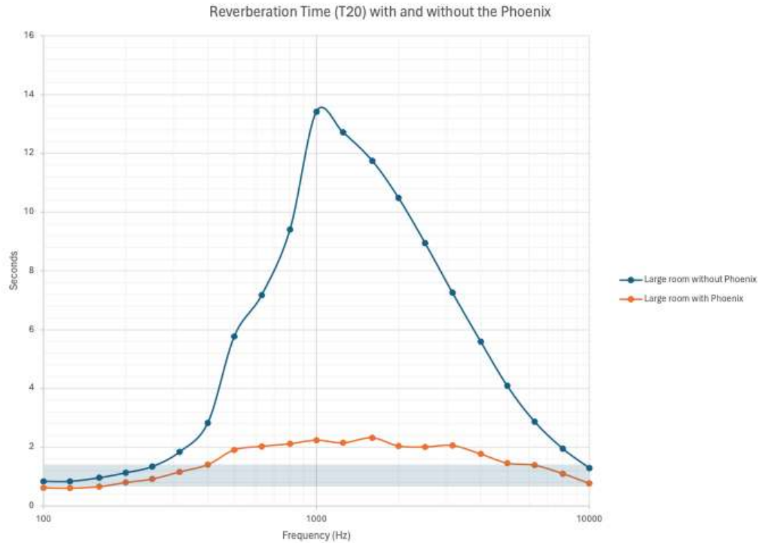
Figure 10. Comparison of T20 of the large gypsum room with and without the Phoenix. The blue box represents recommended reverberation times for rooms for speech and chamber music.
