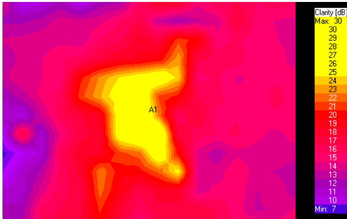
Figure 13. C80 for Large room at \alpha=0.80 .
