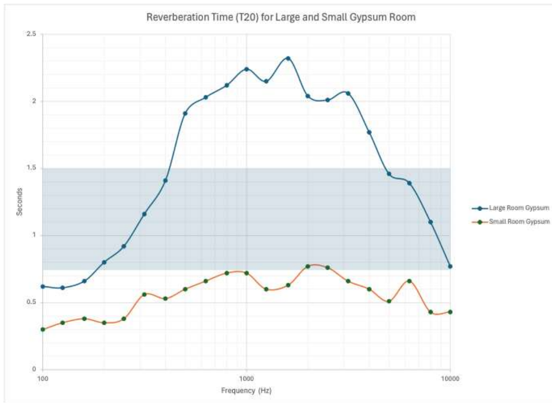
Figure 11. Reverberation time of large and small gypsum room with the Phoenix installed in both. The blue box represents recommended reverberation times for rooms for speech and chamber music.
