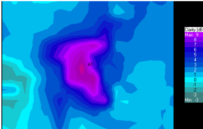
Figure 12. C80 for Large room at \alpha=0.20
