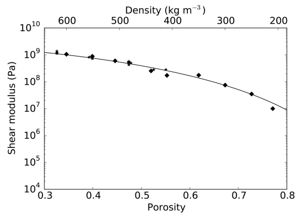
Fig. 3. The shear modulus of snow as a function of porosity (solid line) calculated using Eqns (3–5). Measurements presented by Johnson (1982) and Smith (1969) are indicated with diamonds and stars, respectively.
