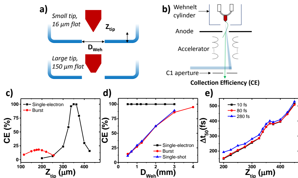
Figure 1. (a) Schematic of the thermionic gun showing the Wehnelt cylinder and LaB 6 with aperture diameter ( D_{Weh} ) and gun-tip height ( Z_{tip} ) defined. (b) Schematic of the thermionic gun geometry in the Tecnai Femto with pertinent components labeled and collection efficiency (CE) illustrated. (c) Effect of Z_{tip} position on CE for the single-electron and burst modes for D_{Weh} = 0.7 mm. (d) Effect of D_{Weh} at optimal Z_{tip} position on CE for each mode studied. (e) Effect of photoelectron-generating laser-pulse duration (10, 80, and 280 fs) on temporal resolution ( \Delta t_{50} ) as a function of Z_{tip} position.
