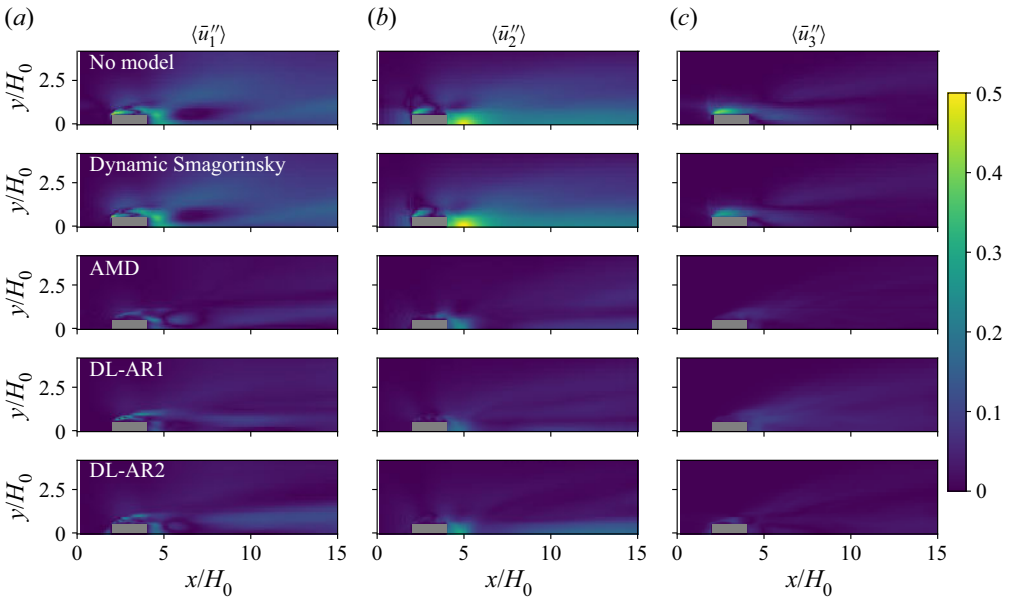
Figure 7. The \ell_1 error for the resolved velocity fluctuations for the AR2 Re_0 = 1000 configuration (ii).
