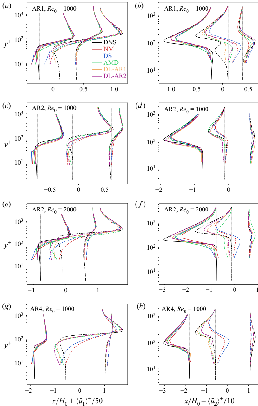
Figure 10. Near-wall streamwise ( a,c,e,g ) and cross-stream ( b,d,f,h ) mean velocity profiles in wall units. Vertical dashed lines indicate x_1 locations. Reference DNS data are plotted on the fine DNS meshes. All lines start at the first mesh node away from the wall.
