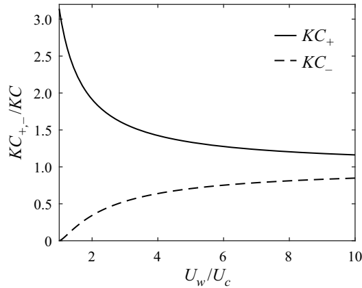
Figure 12. Effective Keulegan–Carpenter numbers, representing flow excursion in the forward (with current) and reverse (against current) directions relative to hemisphere diameter. Effective Keulegan–Carpenter numbers are normalized by KC for the same wave conditions in the absence of current.
