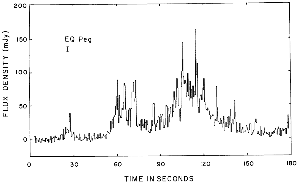
Figure 1. A previously unpublished VLA observation of the total intensity, I , at 1420 MHz (21 cm) from the dwarf M star EQ Pegasi. The flaring emission has a total duration of minutes, with components on shorter time scales of seconds or less. The radiation is up to 100 percent circularly polarized (see Fig. 2).
