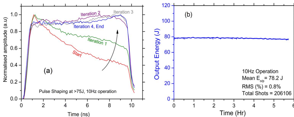
Figure 2. (a) Example of automatic pulse shaping capability of the D100X laser for achieving a flat-top temporal profile at >75 J, 10 Hz operation; (b) long-term stability over 6 h at 10 Hz.
