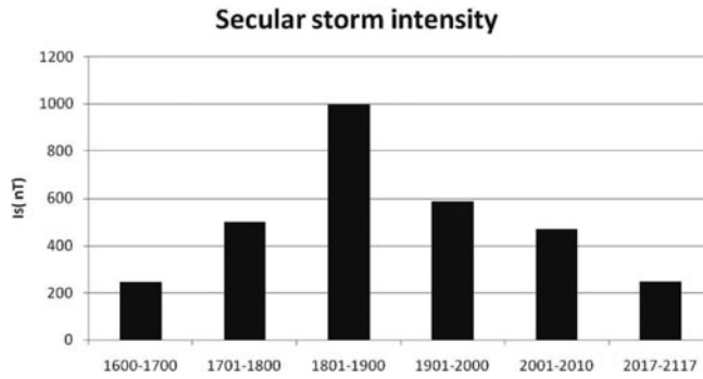
Figure 1. Secular changes in maximum geomagnetic storm intensity ( I_s ) inferred from Aurora and geomagnetic observations for different periods since 17th century. The value for 2017–2117 is only a prediction.
