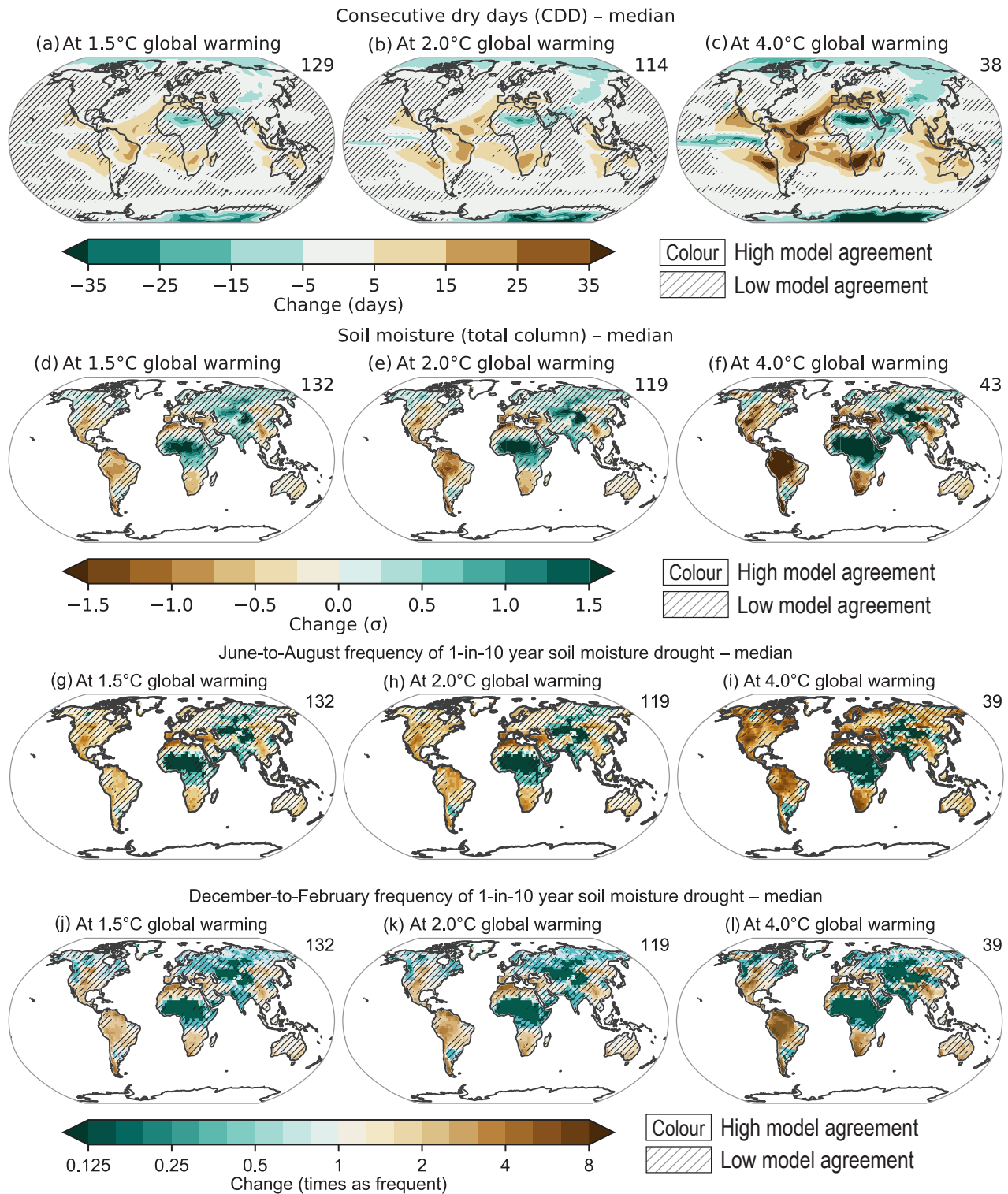
Figure 11.19 | Projected changes in (a–c) the number of consecutive dry days (CDD), (d–f) annual mean soil moisture over the total column, and (g–i) the frequency and intensity of 1-in-10-year soil moisture drought for the June-to-August and December-to-February seasons at 1.5°C, 2°C, and 4°C of global warming compared to the 1850–1900 baseline. The unit for soil moisture change is the standard deviation of interannual variability in soil moisture during 1850–1900. Standard deviation is a widely used metric in characterizing drought severity. A projected reduction in mean soil moisture by one standard deviation corresponds to soil moisture conditions typical of about 1-in-6-year droughts during 1850–1900 becoming the norm in the future. Results are based on simulations from the Coupled Model Intercomparison Project Phase 6 (CMIP6) multi-model ensemble under the Shared Socio-economic Pathway (SSP), SSP1-1.9, SSP1-2.6, SSP2-4.5, SSP3-7.0, and SSP5-8.5 scenarios. The numbers in the top right indicate the number of simulations included. Uncertainty is represented using the simple approach: no overlay indicates regions with high model agreement, where \geq 80\% of models agree on the sign of change; diagonal lines indicate regions with low model agreement, where < 80\% of models agree on the sign of change. For more information on the simple approach, please refer to the Cross-Chapter Box Atlas 1. For details on the methods see Supplementary Material 11.SM.2. Changes in CDDs are also displayed in the Interactive Atlas. Further details on data sources and processing are available in the chapter data table (Table 11.SM.9).
