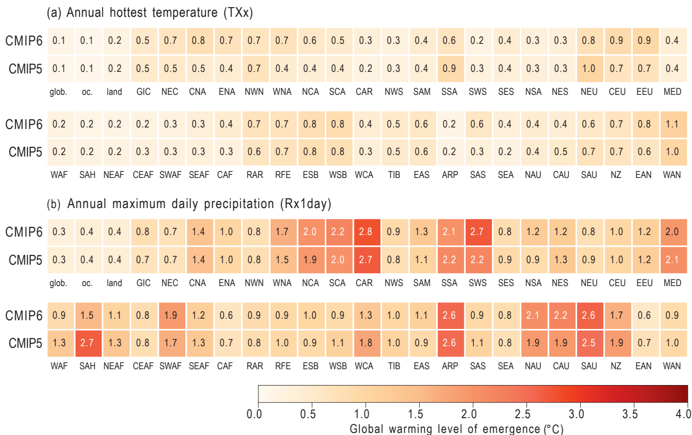
Figure 11.8 | Global and regional-scale emergence of changes in temperature (a) and precipitation (b) extremes for the globe (glob.), global oceans (oc.), global lands (land), and the AR6 regions. Colours indicate the multi-model mean global warming level at which the difference in 20-year means of the annual maximum daily maximum temperature (TXx) and the annual maximum daily precipitation (Rx1day) become significantly different from their respective mean values during the 1850–1900 base period. Results are based on simulations from the Coupled Model Intercomparison Project Phases 5 and 6 (CMIP5 and CMIP6) multi-model ensembles. See Atlas.1.3.2 for the definition of regions. Adapted from Seneviratne and Hauser (2020) under the terms of the Creative Commons Attribution licence.
