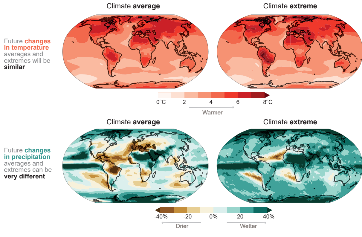
FAQ 11.1, Figure 1 | Global maps of future changes in surface temperature (top panels) and precipitation (bottom panels) for long-term average (left) and extreme conditions (right). All changes were estimated using the Coupled Model Intercomparison Project Phase 6 (CMIP6) ensemble median for a scenario with a global warming of 4°C relative to 1850–1900 temperatures. Average surface temperatures refer to the warmest three-month season (summer in mid- to high latitudes) and extreme temperatures refer to the hottest day in a year. Precipitation changes, which can include both rainfall and snowfall changes, are normalized by 1850–1900 values and shown as a percentage; extreme precipitation refers to the largest daily precipitation in a year.
