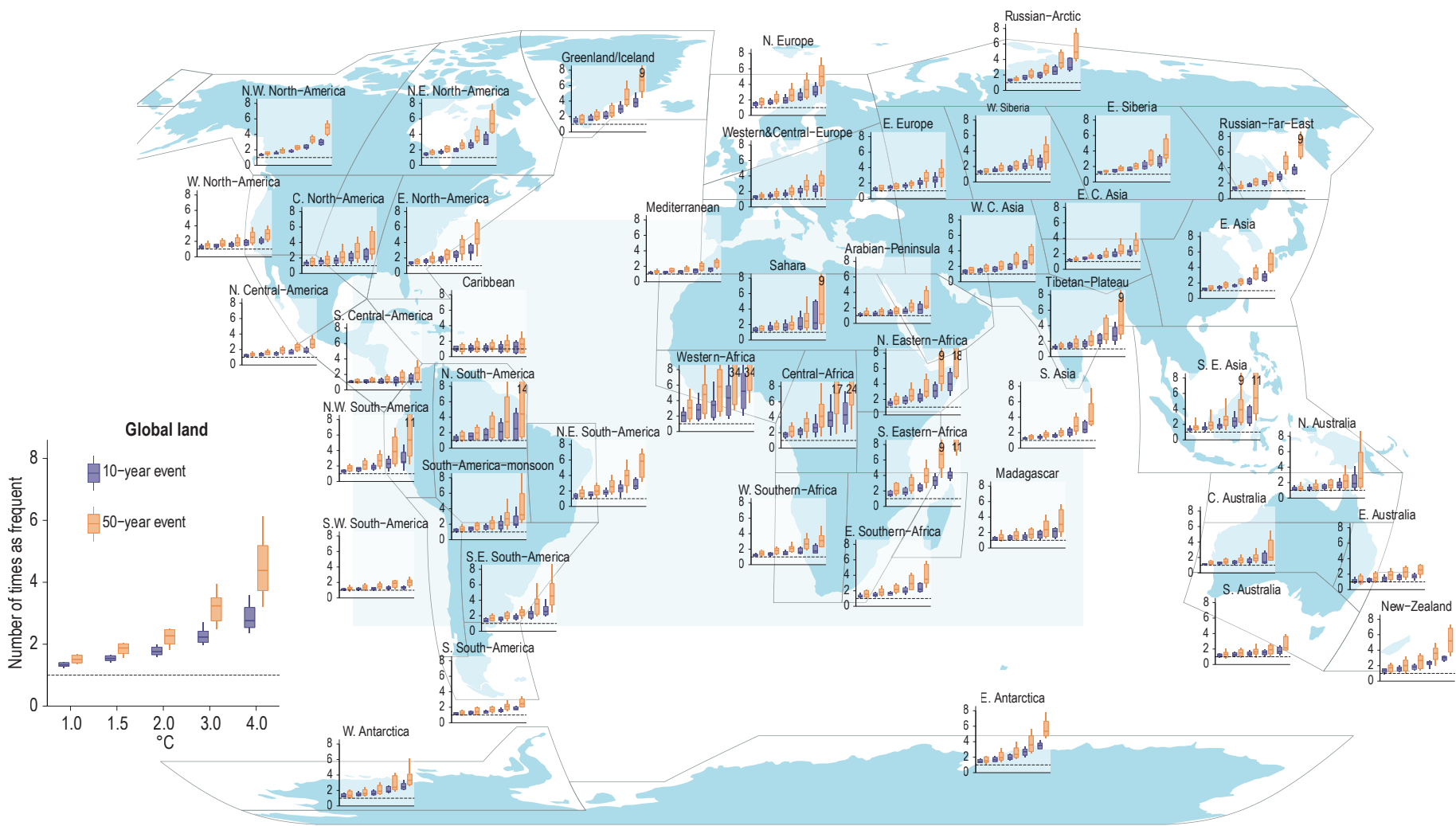
Figure 11.7 | Projected changes in the frequency of extreme precipitation events under 1°C, 1.5°C, 2°C, 3°C, and 4°C global warming levels relative to the 1850–1900 baseline. Extreme precipitation is defined as the annual maximum daily precipitation (Rx1day) that was exceeded on average once during a 10-year period (10-year event, blue) and once during a 50-year period (50-year event, orange) during the 1850–1900 base period. Results are shown for the global land area and the AR6 regions. For each box plot, the horizontal line and the box represent the median and central 66% uncertainty range, respectively, of the frequency changes across the multi-model ensemble, and the ‘whiskers’ extend to the 90% uncertainty range. The dotted line indicates no change in frequency. The results are based on the multi-model ensemble from simulations of global climate models contributing to the Coupled Model Intercomparison Project Phase 6 (CMIP6) under different Shared Socio-economic Pathway forcing scenarios. Adapted from Li et al. (2021). Further details on data sources and processing are available in the chapter data table (Table 11.SM.9).
