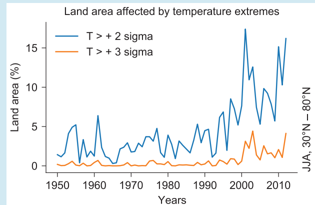
Box 11.4, Figure 1 | Analysis of the percentage of land area affected by temperature extremes larger than two (blue) or three (orange) standard deviations in June–July–August (JJA) between 30°N and 80°N using a normalization. This figure shows a substantial increase in the overall land area affected by very strong hot extremes since 1990. Adapted from Sippel et al. (2015).
