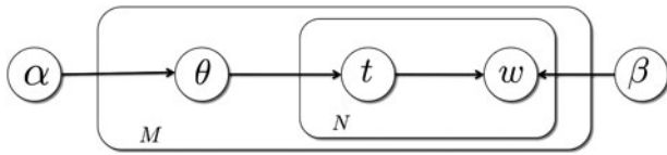
Fig. 1. Graphical representation of the topic model using LDA.
