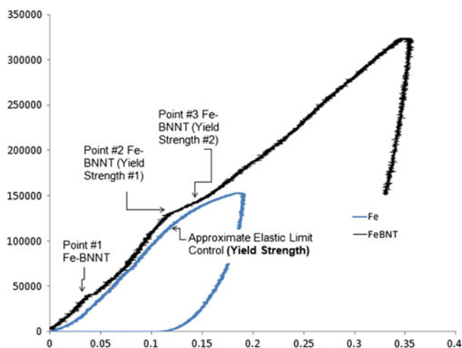
FIG. 2. Specific stress–strain curves of iron–boron nitride nanotube (Fe–BNNT) composite (black) and pure Fe (blue).
