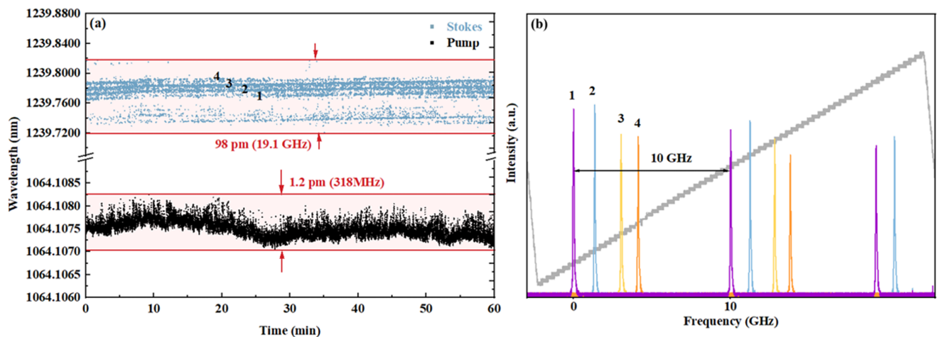
Figure 5. (a) Wavelength stability of the Stokes and pump outputs for 1 hour. (b) Four typical FPI traces of the SLM Stokes output after multiple acquisitions.
