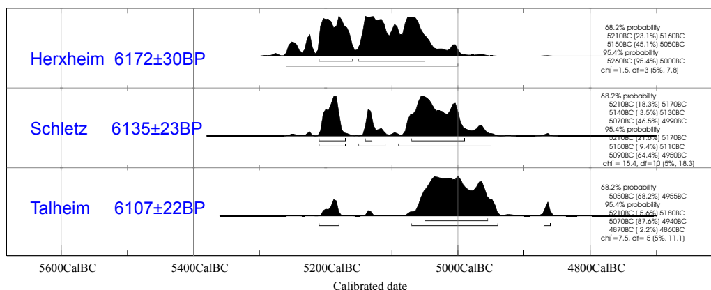
Figure 4 Calibration of the mean 14 C age values from the 3 sites investigated in this study. The results of the χ 2 are also listed.
