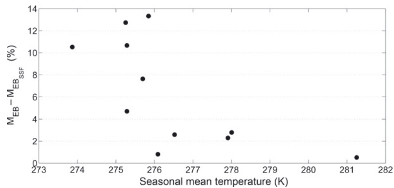
Fig. 2. Difference in total melt at the end of the season computed by EB ( M_{EB} ) and EB SSF ( M_{EB_{SSF}} ) versus mean temperature over the season for all sites investigated. The difference is expressed as % over the total simulated by EB.
