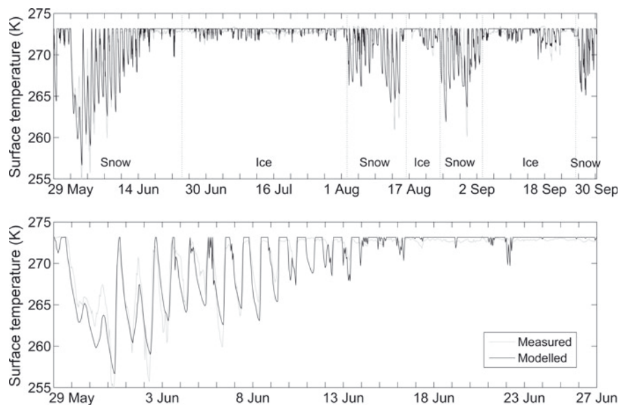
Fig. 4. Comparison of measured and simulated surface temperature at Haut Glacier d'Arolla lowest station in 2006 for the entire ablation season (top) and for the snow-covered period, 28 May to 27 June (bottom). Simulated temperature is obtained with EB SSF .
