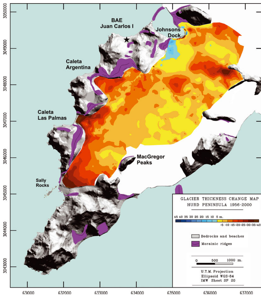
Fig. 4. Map of ice-thickness change, 1956–2000. The area located between the 1956 and 1999/2000 ice fronts was not surveyed and is shown in white. Moraines on the proglacial areas are displayed to show earlier Holocene glacier margin positions.
