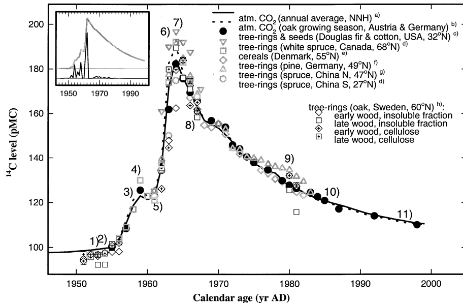
Figure 1 The bomb-pulse curve. a) The annually averaged atmospheric ^{14}\text{CO}_2 curve for the 30^\circ\text{--}90^\circ\text{N} latitude band provided by I Levin (personal communication). b) Atmospheric ^{14}\text{CO}_2 data from Vermont, Austria ( 47^\circ\text{N} ) and Schauinsland, Germany ( 48^\circ\text{N} ) (Levin et al. 1997) but only averaged for April to August, the growing season of oaks (Rom 2000). c) See Table 1. d) Trees from the Mackenzie Delta, Canada, and Mingyin, Yunnan Province, China (Dai and Fan 1986). e) Mainly ears (but also grains or green parts) of barley, wheat, rye and oats from the Copenhagen area (Tauber 1967). Note that the (annually averaged) values given are only approximate values since the original data had been published as D using a physical ^{14}\text{C} half-life of 5570 yr and 1958 as the reference year. Regarding the rather high value for 1959 Tauber (1967) mentions that in that year the polar front had an extreme northern position at European latitudes during the whole summer. f) Tree from Obrigheim, Germany (Levin et al. 1985). g) Tree from Dailing, Heilongjiang Province, China (Dai et al. 1992). h) Different sections and different chemical fractions in tree-rings from an oak from Uppsala, Sweden (Olsson and Possnert 1992).
