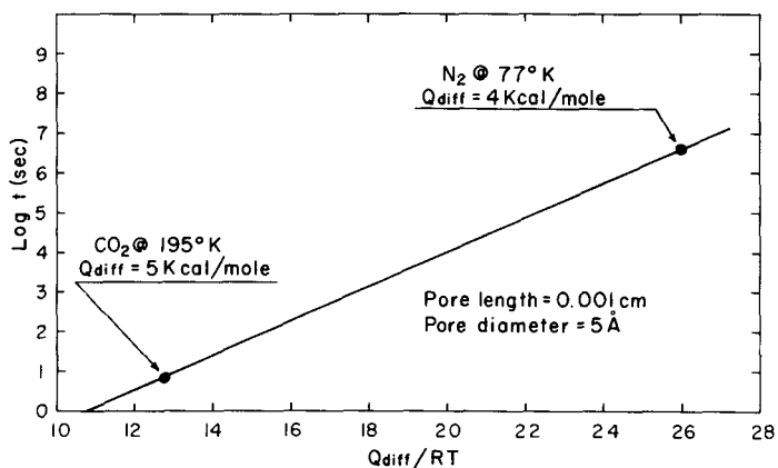
Fig. 1. Plot showing the time of passage ( t ) of a gas molecule as a function of the reduced differential heat of adsorption ( Q_{diff} ).
