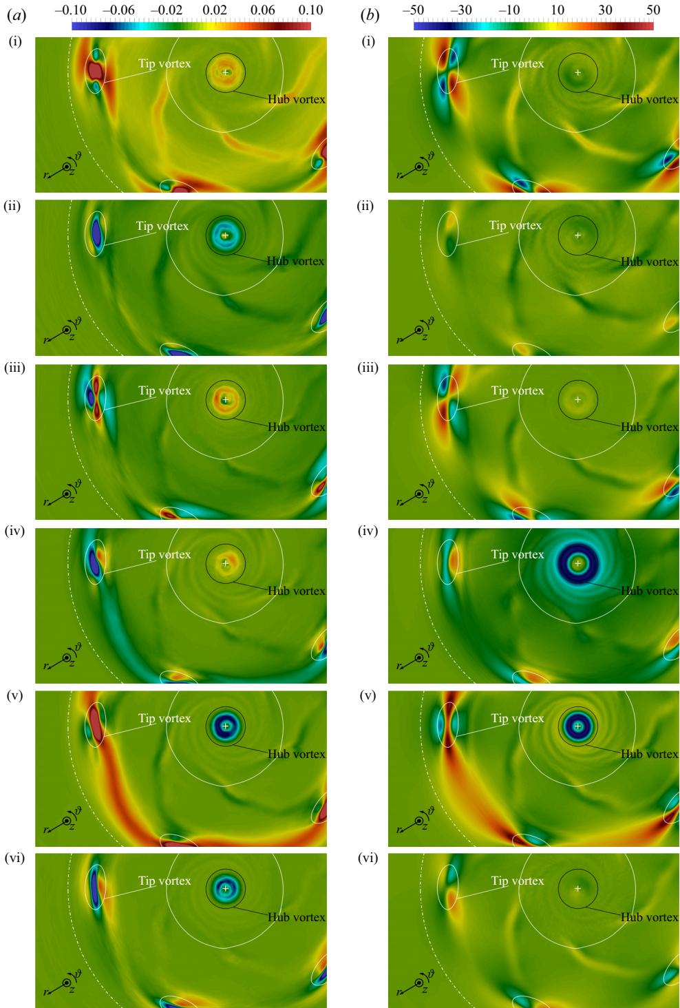
Figure 26. Contours of (a) \hat{R}_{ij}^d and (b) -\hat{S}_{ij} from phase-averaged statistics at the working condition J4 . Components of the tensors, scaled by U_\infty^2 and U_\infty/D , respectively, at the streamwise coordinate z/D = 1.0 : (i) rr ; (ii) r\vartheta ; (iii) zz ; (iv) r\vartheta ; (v) rz ; (vi) \vartheta z . White and black isolines of pressure coefficients \hat{c}_p = -2.0 and \hat{c}_p = -10 , respectively. Dotted-dashed line encompassing the projection of the area swept by the propeller.
