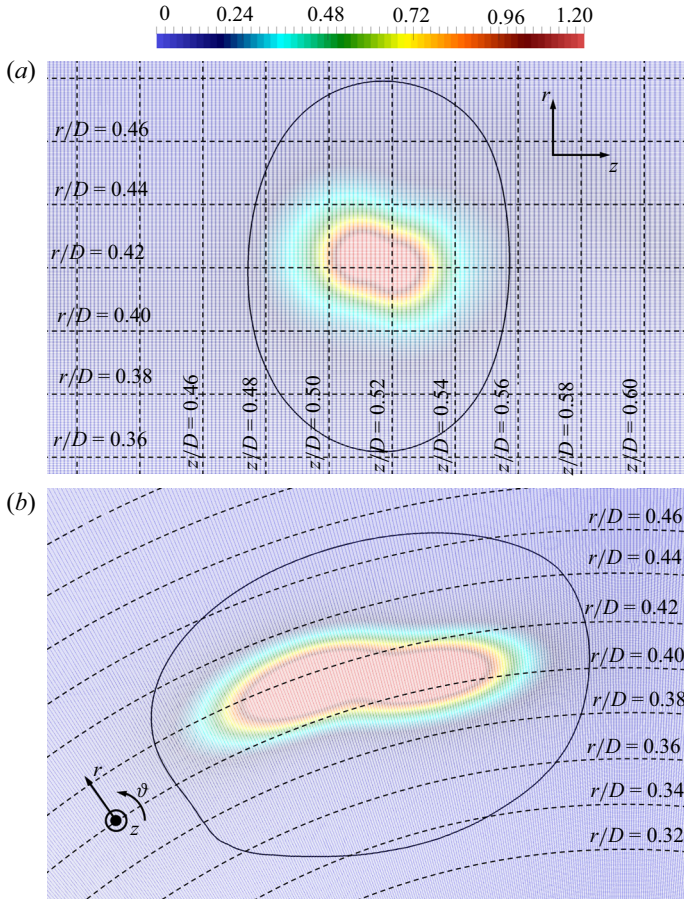
Figure 11. Contours of phase-averaged root-mean-squares of the fluctuations of pressure coefficient at the working condition J_4 : (a) detail on the meridian plane of figure 10(e) at z/D \approx 0.5 ; (b) detail on the cross-stream section at z/D = 0.5 . Black isolines of phase-averaged pressure coefficient \hat{c}_p = -0.6 isolating the core of the tip vortices. Grid points shown to visualize the resolution of the computational grid within the tip vortices.
