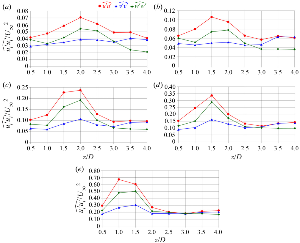
Figure 14. Streamwise evolution of the phase-averaged normal, turbulent stresses at the core of the tip vortices in the radial ( \widehat{u'u'} ), azimuthal ( \widehat{v'v'} ) and axial ( \widehat{w'w'} ) directions, respectively. Comparison across advance coefficients: (a) J0 ; (b) J1 ; (c) J2 ; (d) J3 ; (e) J4 . Note the variation of the vertical scale across panels.
