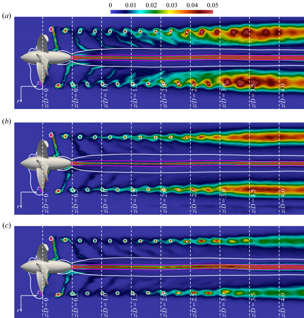
Figure 15. Contours of phase-averaged normal, turbulent stresses at the working condition J_0 , scaled by U_\infty^2 : (a) radial, \overline{u'u'} ; (b) azimuthal, \overline{v'v'} ; (c) axial, \overline{w'w'} . White and magenta isolines of pressure coefficients \hat{c}_p = -0.4 and \hat{c}_p = -2.0 , respectively.
