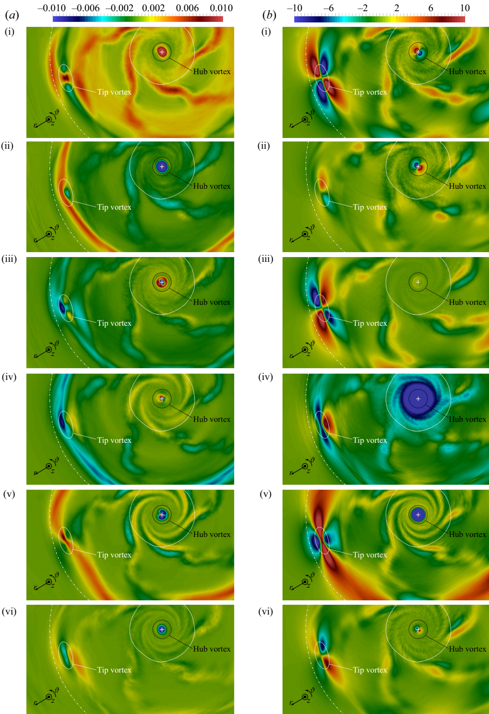
Figure 24. Contours of (a) \hat{R}_{ij}^d and (b) -\hat{S}_{ij} from phase-averaged statistics at the working condition J_0 . Components of the tensors, scaled by U_\infty^2 and U_\infty/D , respectively, at the streamwise coordinate z/D = 1.0 : (i) rr ; (ii) r\vartheta ; (iii) zz ; (iv) r\vartheta ; (v) rz ; (vi) \vartheta z . White and black isolines of pressure coefficients \hat{c}_p = -0.4 and \hat{c}_p = -2.0 , respectively. Dotted-dashed line encompassing the projection of the area swept by the propeller.
