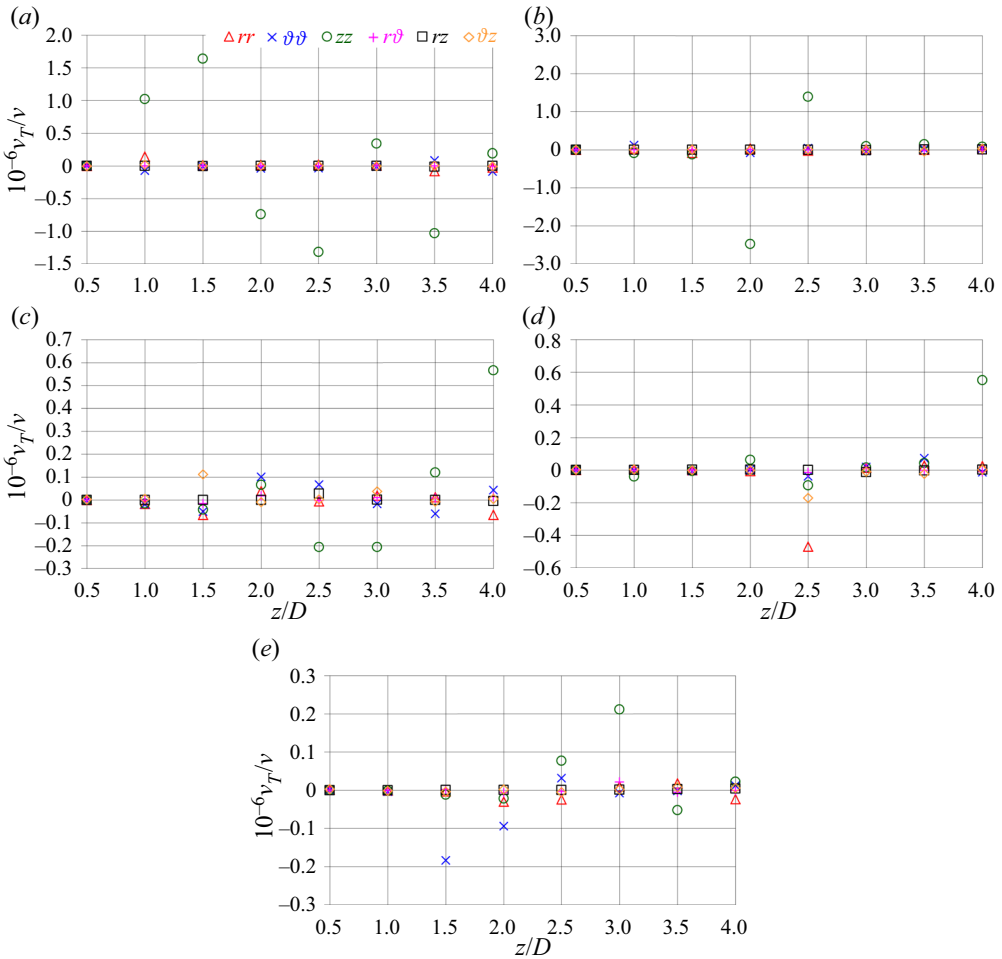
Figure 27. Turbulent viscosity, computed as in (4.5), at the core of the hub vortex. Comparison across advance coefficients: (a) J0 ; (b) J1 ; (c) J2 ; (d) J3 ; (e) J4 . Note the variation of the vertical scale across panels.
