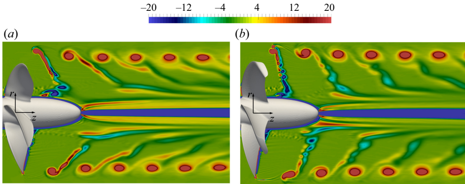
Figure 33. Contours of phase-averaged azimuthal vorticity, scaled by U_\infty/D , on a meridional plane: near wakes of the (a) conventional and (b) tip-loaded propellers.
