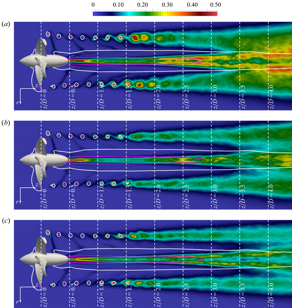
Figure 17. Contours of phase-averaged normal, turbulent stresses at the working condition J4 , scaled by U_{\infty}^2 : (a) radial, \overline{u'u'} ; (b) azimuthal, \overline{v'v'} ; (c) axial, \overline{w'w'} . White and magenta isolines of pressure coefficients \hat{c}_p = -2.0 and \hat{c}_p = -10 , respectively.
