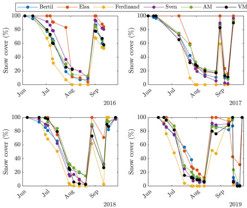
Fig. 2. Snow cover dynamics on the selected glaciers expressed as a percentage during the summer ablation seasons for the period 2016–19.
