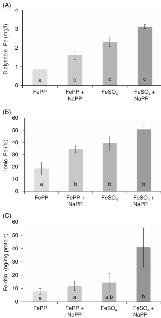
Fig. 2. Results of the in vitro experiments for the four different bouillons containing either ferric pyrophosphate (FePP) only, FePP+tetra sodium pyrophosphate (NaPP), ferrous sulphate (FeSO 4 ) only or FeSO 4 +NaPP. Bars represent dialysable (A) and ionic Fe (B) from simulated gastric and small intestinal digestion and ferritin response (C) from Caco-2-cell assay. Error bars with whiskers indicate standard deviations ( n 3). a,b,c Mean values with unlike letters were significantly different in a one-way ANOVA followed by Bonferroni correction for multiple comparison ( P < 0.05).
