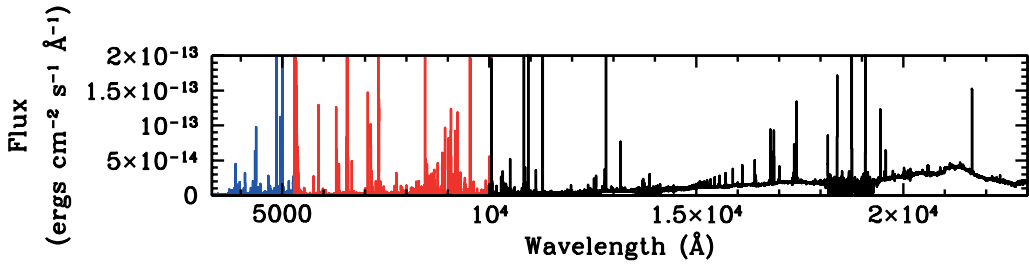
Figure 1. X-shooter spectrum of the core of M2-9 with UVB (blue), VIS (red) and NIR (black) spectra overlaid.
