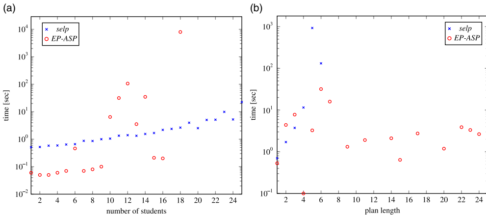
Fig. 2. Benchmark results. Missing points indicate timeouts.
