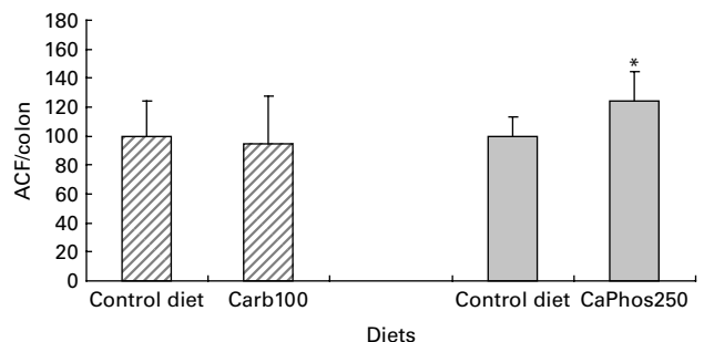
Fig. 4. Effect of calcium salts in diet on putative precancerous lesions (aberrant crypt foci (ACF)) per rat colon 101 d after the injection of dimethylhydrazine. Results of the present study with 100 µmol/g calcium carbonate are represented by ▨. Results of the previous study with 250 µmol/g calcium phosphate (Pierre et al. (16) ) are represented by ▩. Results are expressed after normalisation of the control diet groups to 100. * Mean values were significantly different control group. Note: the control diet was a low-Ca Hb diet supplemented with calcium carbonate at 33 µmol/g. Carb100 and CaPhos250 are low-Ca Hb diets supplemented, respectively, with calcium carbonate (100 µmol/g) and calcium gluconate (230 µmol/g).
