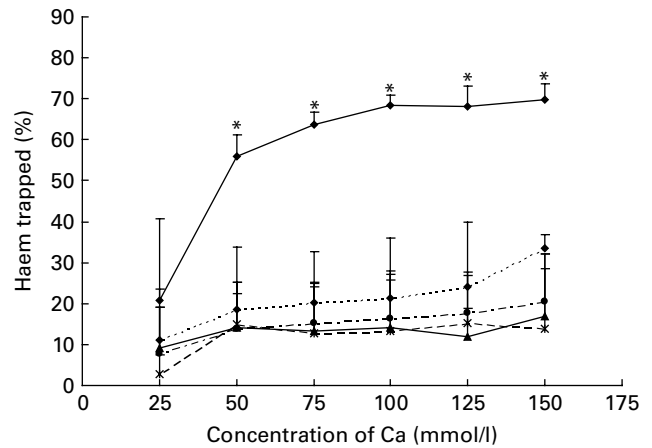
Fig. 2. Effect of Ca salts on haem solubility in vitro . Haem (0.36 mM) was incubated with six different concentrations of Ca salts (150, 125, 100, 75, 50 and 25 mmol/l). Data are means, and bars are standard deviations ( n = 3 ). * Mean values were significantly different from other salts. —◆—, Calcium carbonate; —●—, calcium phosphate; —▲—, calcium chloride; —●—, calcium gluconate; —✱—, calcium lactate.
