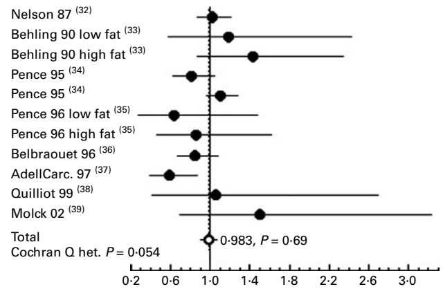
Fig. 5. Meta-analysis of the relation between calcium carbonate and colon cancer in carcinogen-injected rats. The common relative risk with 95% CI was calculated from eleven studies. The study-specific relative risk is represented by ●. The common relative risk is represented by ○. Horizontal lines are 95% CI. References are indicated between brackets. Het., heterogeneity.
