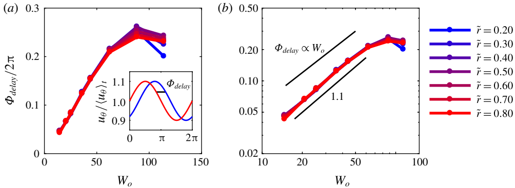
FIGURE 5. (Colour online) The delay between the driving modulation and the fluid velocity response as a function of Womersley number Wo . The delay \Phi_{delay} is normalized with 2\pi of the modulation. The phase delay is calculated for a number of radii, not showing much difference. The same data are shown in linear scale (a) and logarithmic scale (b). The results are radially binned within \tilde{r} \pm 0.025 . The inset in (a) shows how the phase delay \Phi_{delay} is defined: \Phi_{delay} is calculated by cross-correlating both signals. We included the scaling of the response for laminar flow, which equals \Phi_{delay} \propto Wo .
