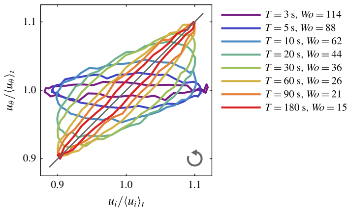
FIGURE 3. (Colour online) Phase-averaged normalized azimuthal mid-gap flow velocity u_\theta/\langle u_\theta \rangle_t as a function of normalized driving velocity of the inner cylinder u_i/\langle u_i \rangle_t . We show the result for all measured Womersley numbers Wo . The velocity is radially averaged between 0.3 \leq \tilde{r} \leq 0.7 . The solid grey line corresponds to the quasi-stationary case u_\theta/\langle u_\theta \rangle_t = u_i/\langle u_i \rangle_t . The arrow at the bottom right indicates the direction of the cycles.
