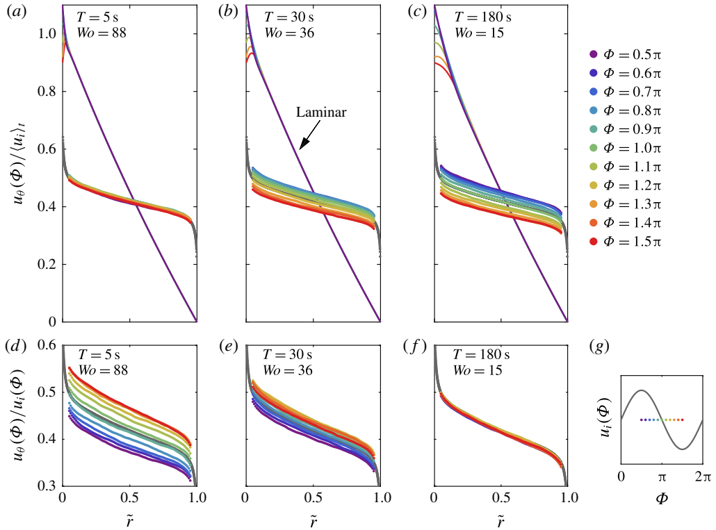
FIGURE 4. (Colour online) Azimuthal velocity profiles as a function of dimensionless radius \tilde{r} . All data are phase-averaged and normalized. (a–c) Here u_\theta(\Phi) is normalized with the time-averaged inner cylinder velocity \langle u_i \rangle_t = 6.3 \text{ m s}^{-1} , i.e. the same constant value for all lines. A collapse of all lines indicates that the response amplitude is small, as is observed for large Wo (see panel (a)). Furthermore, we show the response of laminar flow to the modulation, calculated numerically (see § 2). (d–f) Here u_\theta(\Phi) is normalized by the instantaneous inner cylinder velocity at phase \Phi , i.e. u_i(\Phi) (a value between u_i(0.5\pi) = 6.9 \text{ m s}^{-1} and u_i(1.5\pi) = 5.7 \text{ m s}^{-1} ). A collapse of all lines indicates that the behaviour of the system is quasi-stationary, as can be seen for small Wo in panel (f). The solid grey lines show the azimuthal velocity profile for Re_i = 5 \times 10^5 for the non-modulated, stationary case (data from Huisman et al. (2013b)). (g) The azimuthal velocity u_\theta(\Phi) is shown for a series of phases of the modulation; here we show data for phases between 0.5\pi \leq \Phi \leq 1.5\pi , i.e. half of a modulation cycle, as shown in this inset. See also figure 2 for the definition of phase \Phi .
