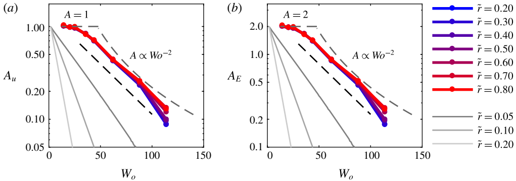
FIGURE 6. (Colour online) Amplitude response as a function of the Womersley number Wo for various dimensionless radii. The coloured lines represent our measurements, and the solid grey lines are numerically calculated laminar flow responses. (a) The response amplitude of the velocity A_u and (b) the response amplitude of the energy A_E . The experimental results are radially binned between \tilde{r} \pm 0.025 . The dashed grey lines show the scalings of A as predicted by von der Heydt et al. (2003a). We included the laminar responses, shown in solid grey lines. A number of radii are included, to highlight the dependence on the radius, which does not exist in the well-mixed turbulent case. The effective slope of the measurements A \propto e^{-0.025Wo} is shown in dashed black. This would correspond to the slope of the laminar flow response at \tilde{r} \approx 0.035 .
