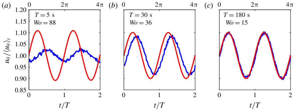
FIGURE 2. (Colour online) Normalized azimuthal velocity of the sinusoidally driven inner cylinder u_i/\langle u_i \rangle_t (solid red) and normalized azimuthal velocity u_\theta/\langle u_\theta \rangle_t at mid-gap (solid blue). Three Womersley numbers are shown, (a) Wo = 88 , (b) Wo = 36 and (c) Wo = 15 . The velocity is radially averaged between 0.3 \leq \tilde{r} \leq 0.7 . On the top x -axis, we show the phase \Phi of the modulations in radians.
