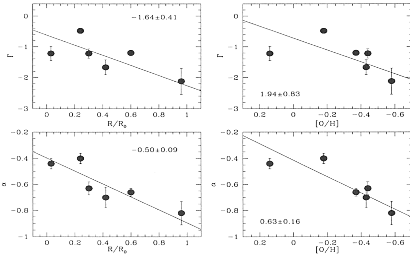
Figure 2. Relations among \alpha (the slope of the luminosity function), \Gamma (the slope of the stellar IMF), [O/H] (the abundance derived from the H II regions), and the galactocentric distance of the clusters in M33. The solid lines represent linear fits to the data.
