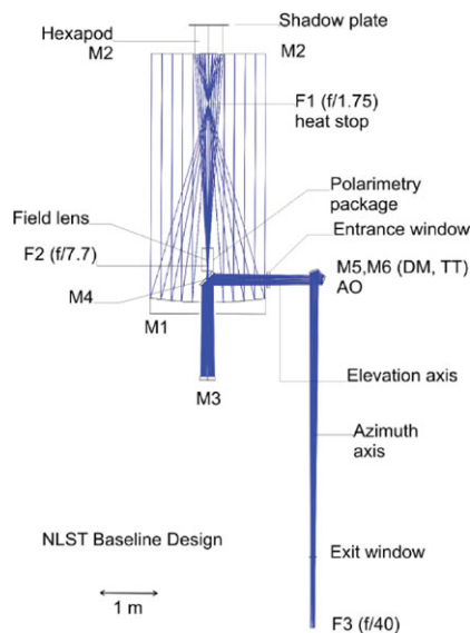
Figure 1. Optical layout of NLST
