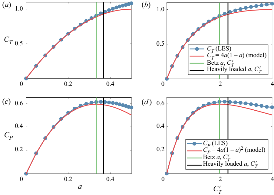
Figure 11. Comparison between yaw-aligned ( \gamma = 0 ) momentum theory and LES results for the ADM without the disk velocity u_d correction factor ( M = 1 , \Delta/D = 0.29h/D = 0.032 ). For a yaw-aligned turbine, the rotor-normal induction is a_n = a , where a is the standard axial induction factor predicted by momentum theory. Coefficient of thrust C_T is shown as a function of (a) induction factor a , and (b) C'_T . Coefficient of power C_P is shown as a function of (c) induction factor a , and (d) C'_T . The vertical lines report the induction a and thrust coefficient C'_T corresponding to the Betz limit ( a = 1/3 , C'_T = 2 ) and the heavy loading limit ( a = 0.37 , C'_T = 2.3 ) (Wilson & Lissaman 1974; Burton et al. 2011).
