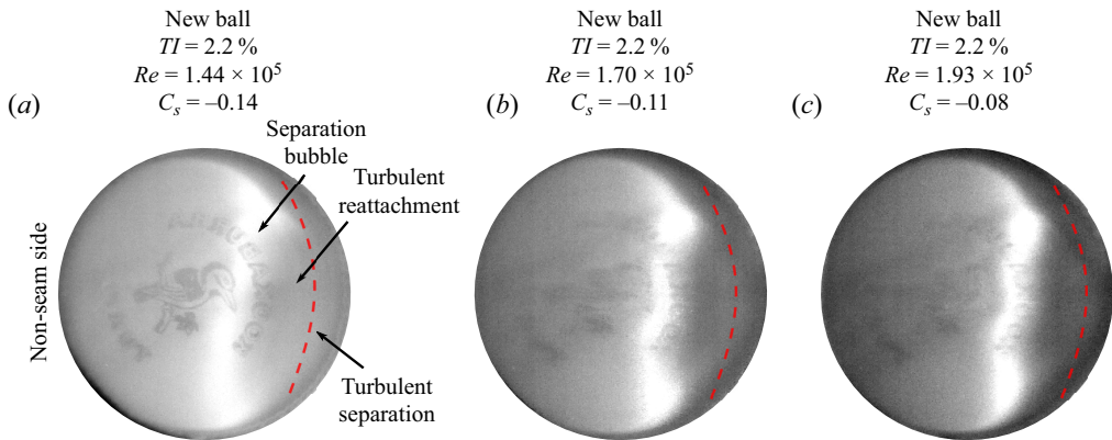
Figure 23. Non-seam side IR image of a new cricket ball with grid-generated turbulent intensity of 2.2% for varying Re . Flow is left to right and red dashed lines illustrate eventual separation position.
