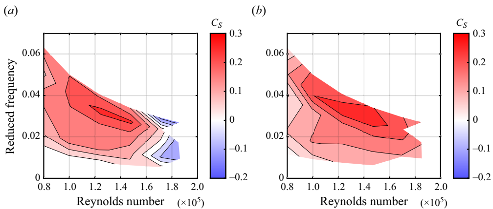
Figure 19. Swing force coefficient, C_S , against Reynolds number, Re , and reduced frequency reprocessed in non-dimensional form from data presented in Bentley (1982) for two balls at seam angle 20^\circ with (a) ball 8 and (b) ball 11.
