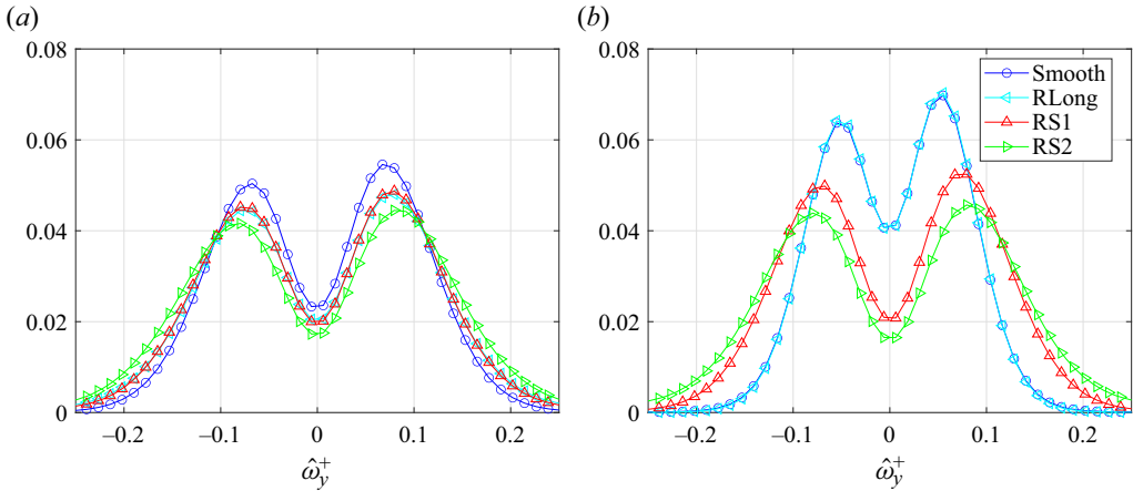
Figure 6. Probability density functions of the wall-normal vorticity \hat{\omega}_y^+ calculated at the streaks' edges. Data are collected at (a) Re_\theta = 2200 and y^+ = 35 , (b) Re_\theta = 2900 and y^+ = 50 .
