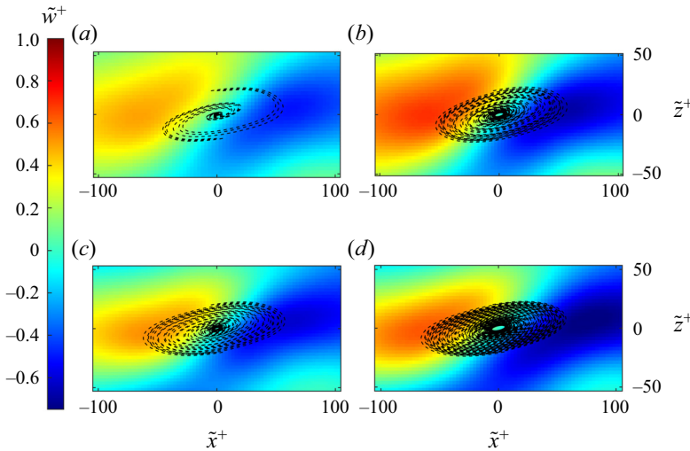
Figure 11. VISA conditionally averaged spanwise velocity ( \tilde{w}^+ ) for events characterized by \partial u/\partial x < 0 and \partial u/\partial z > 0 , with overlaid streamlines, for cases (a) Smooth, (b) RLong, (c) RS1, and (d) RS2. Data are collected at Re_\theta = 2900 and y^+ = 50 .
