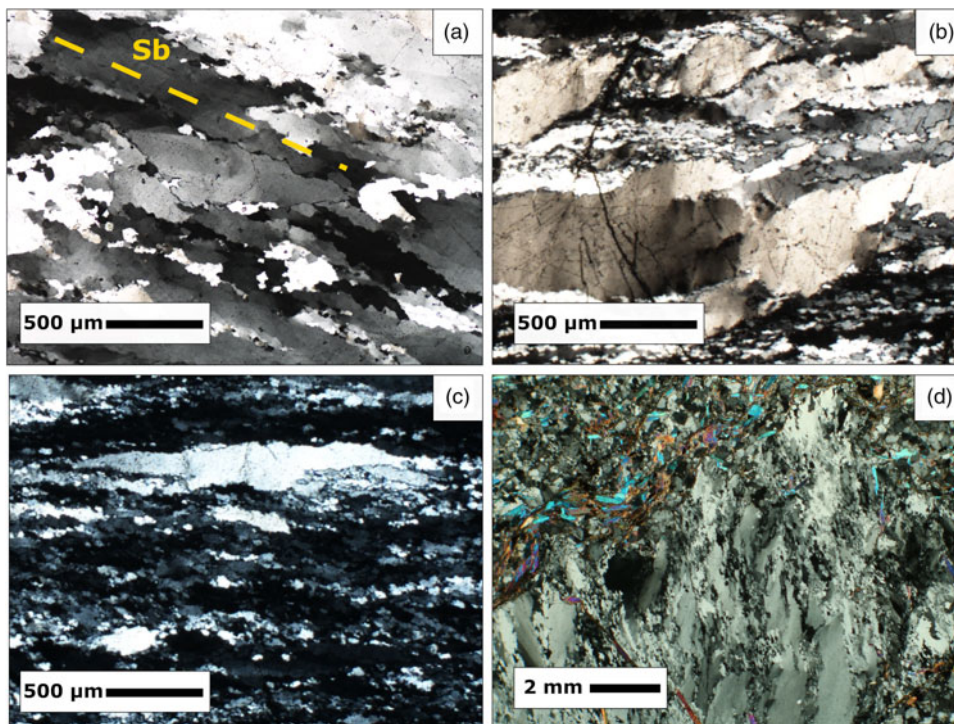
Fig. 5. (Colour online) General overview of syn-D2 quartz microstructures recognized in the study area along samples collected at different distances from the high strain zone of the PAL (i.e. boundary between L-MGMC and HGMC). (a) Southern sector of the study area: quartz microstructures are dominated by GBM recrystallization with incipient SGR. Sb represents the oblique foliation due to the shape preferred orientation (SPO) of quartz aggregates (crossed nicols). (b) Central sector of the study area: SGR microstructures are more developed (crossed nicols). (c) In the northern sector of the study area, close to the high strain zone, the SGR process is pervasive and completely obliterates GBM microstructures (crossed nicols). (d) Plastic deformation in quartz within the hinge zone of an F3 fold where the SPO of quartz crystals is parallel to the S3 foliation (crossed nicols).
