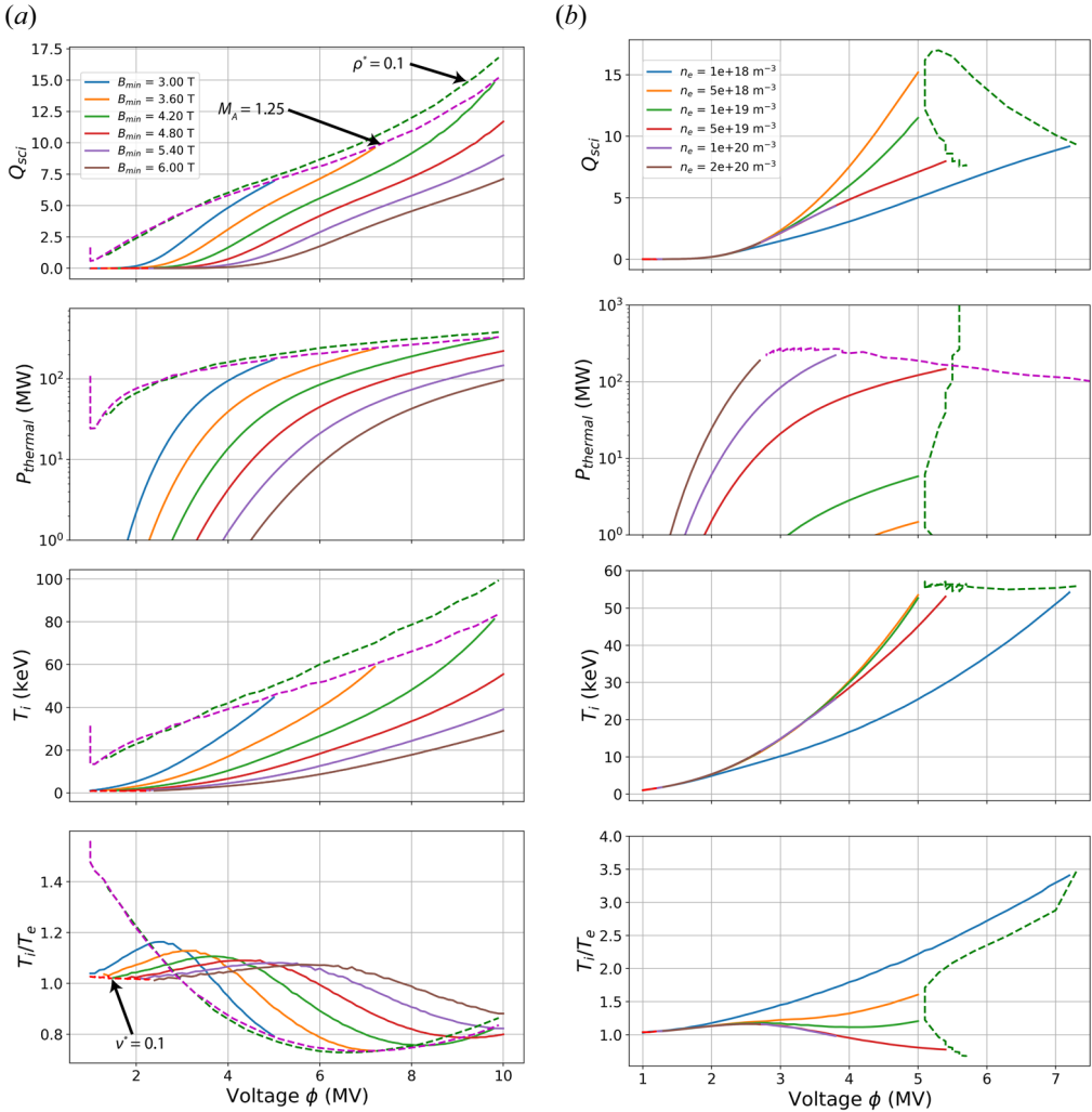
FIGURE 6. Performance of a reactor-like device for 18 T throat field with (a) a range of central fields ( B_{min} ) and fixed electron density ( n_e = 9 \times 10^{19} \text{ m}^{-3} ) and (b) a range of electron densities ( n_e ) and fixed central field ( B_{min} = 5 \text{ T} ). Results were cut off above the values of M_A > 1.25 and \rho^* > 0.1 , indicated by the magenta and green dashed lines, respectively, and where appropriate.
