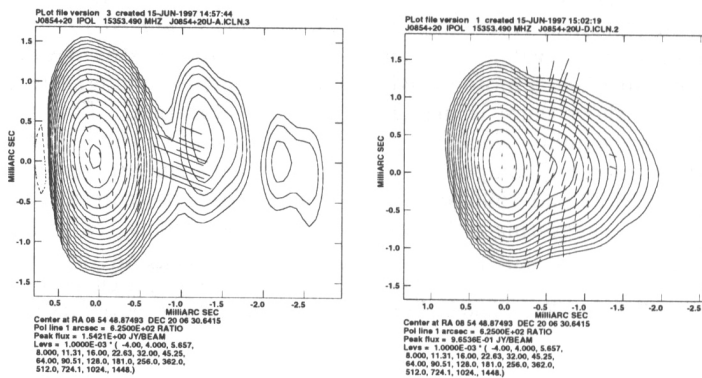
Figure 2. 15 GHz VLBA images of OJ 287, epochs 1996.05 (left) and 1996.58 (right). Contours are logarithmic and indicate total intensity. The ticks indicate the direction of the electric field vectors. The length of the ticks are proportional to the fractional polarization.
