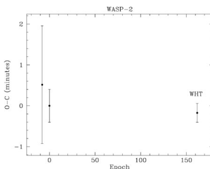
Figure 3. O-C residuals of mid-transit times of WASP-2 system show the resulting transit time is consistent with the ephemeris given in Charbonneau et al. (2007).
