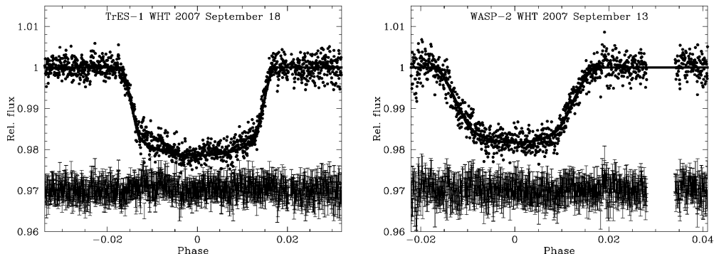
Figure 1. Relative photometry for TrES-1 (left) and WASP-2 (right) is shown with the best-fitting model (solid line). The residuals and rescaled 1\sigma error bars are also plotted, offset by a constant flux for clarity.
