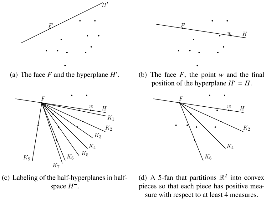
Figure 3. An example of a fan partition of \mathbb{R}^2 for n = 5 and c = 4 .
