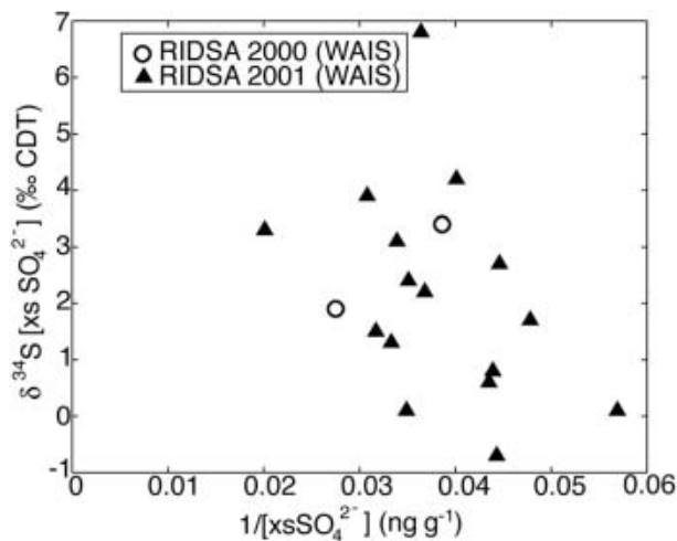
Fig. 4. The \delta^{34}\text{S} measurements for the \text{xsSO}_4^{2-} portion of the total sulfate from the RIDSA core plotted against the inverse of the \text{xsSO}_4^{2-} concentration.
