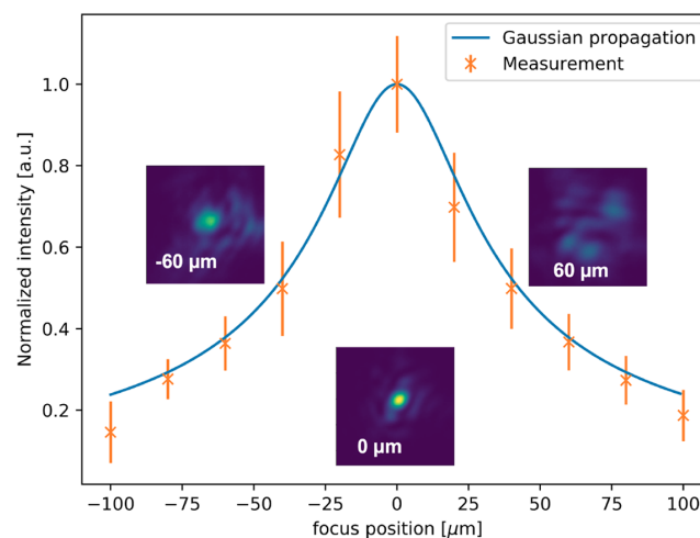
Figure 8. Laser focal spot measured with the focal spot diagnostic. A defocus scan is shown as well as the typical far-field for three positions. The colour scale at 0 \mu\text{m} has been reduced by 2.3\times compared with the other far-fields for visibility.
