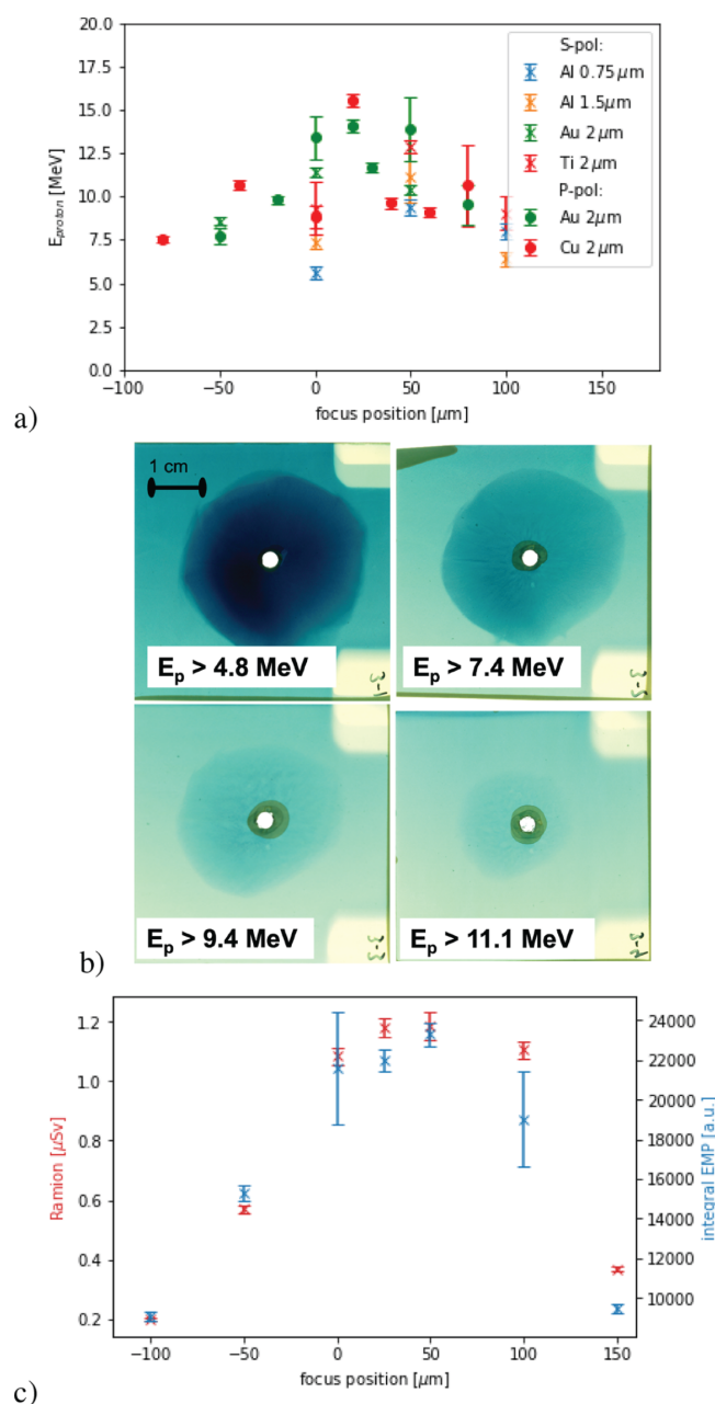
Figure 11. (a) Maximum proton energies as a function of defocusing distance. (b) RCF raw images of the proton beam. (c) Secondary radiation dose measured by a Ram Ion and integral of the EMP spectrum as a function of focal distance for a 2 \mu\text{m} Ti target.
