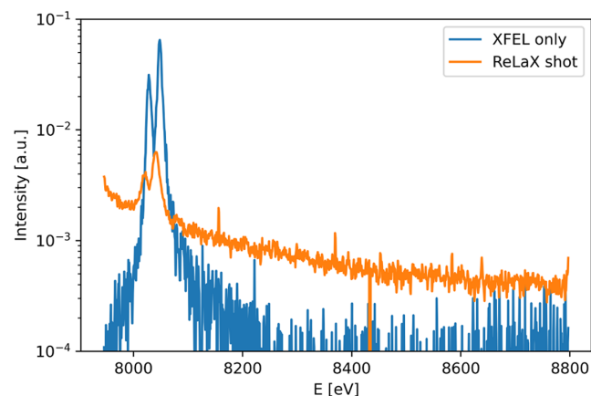
Figure 17. Normalized intensity of the recorded X-ray spectra.
