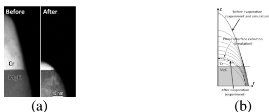
Fig. 1: (a) scanning transmission electron microscopy (STEM) side view of the tested specimen before and after evaporation, (b) Comparison between the simulation results and the observation of the experiment.
