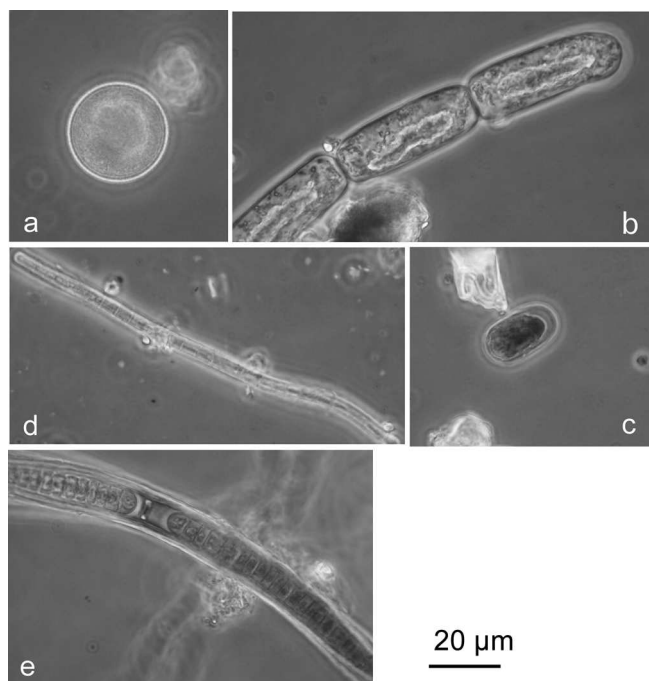
Fig. 3. Photographs of the snow algae observed on Akkem glacier: (a) Chloromonas sp.; (b) Ancydonema nordenskiöldii ; (c) Mesotaenium breggrenii ; (d) Oscillatoriaceae cyanobacterium; and (e) Calothrix parietina . All photographs were taken with a phase-contrast microscope. All samples were stored at -10^{\circ}\text{C} before microscopy, so some cell structure may be broken.
