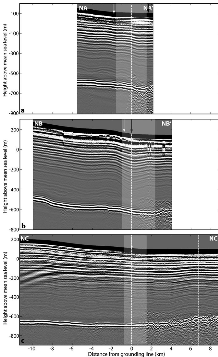
Fig. 2. 3 MHz radar profiles across the northern grounding line of SDM. Data in the upper ~50 m (shown as a black band) are obscured by the direct wave from the transmitter. In all profiles, ice flows from left to right. Black arrow indicates the location of the stratigraphic syncline (described in text). The coupling line or slope break is indicated by the white arrow, and hydrostatic equilibrium is met at the grounding line which is located at km 0. Error in the grounding line position is shown as a transparent white box. (a) Profile NA–NA'. (b) Profile NB–NB'. (c) Profile NC–NC'. In (c), data extend far enough from the grounding line to cross the second hydrostatic line (Vaughan, 1995).
