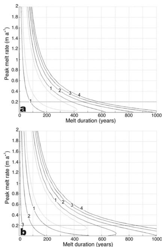
Fig. 6. Model misfit for dipping internal layers across the north SDM grounding line. Contours represent solutions for J=0.5, 1, 2, 3 and 4. Results for (a) profile NA–NA' and (b) profile NB–NB'. Dashed line at 0.2 \text{ m a}^{-1} represents predicted melt rate by Holland and others (2003).
