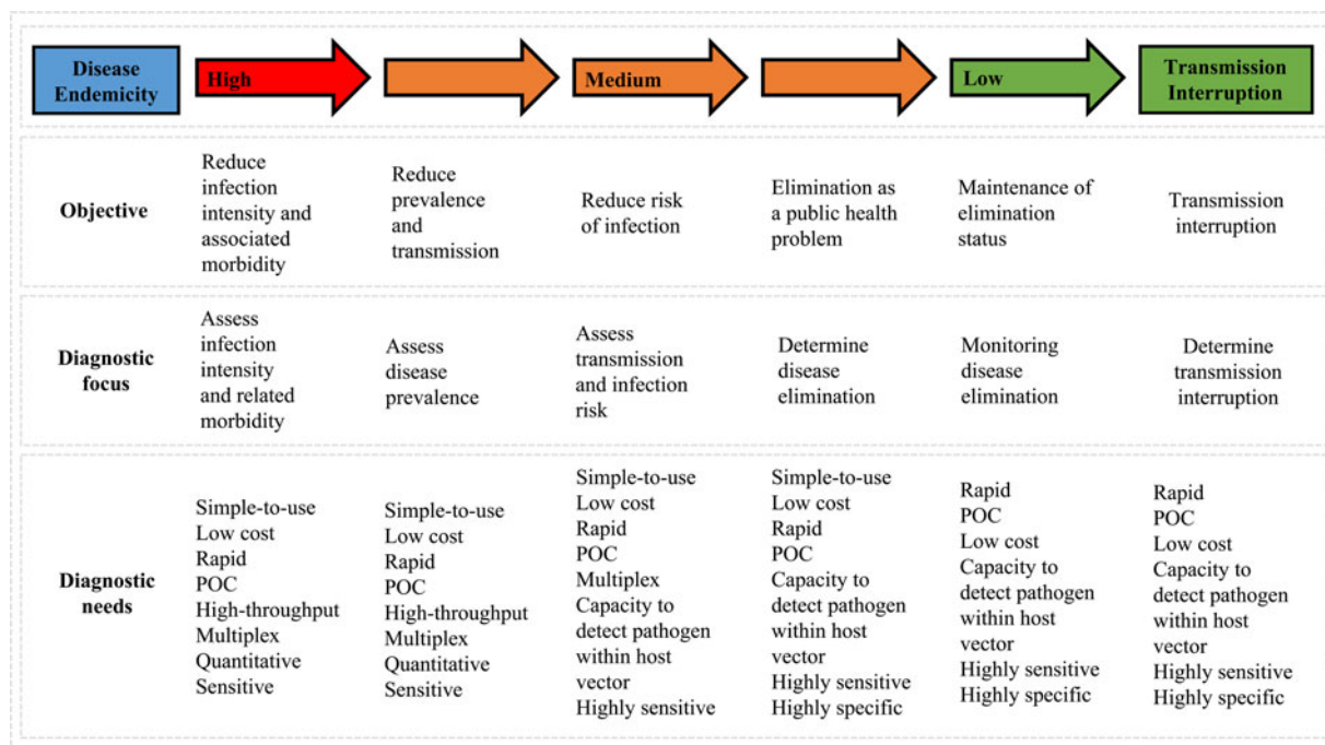
Fig. 1. Schematic outlining changes in diagnostic priorities as control programmes progress (adapted from Bergquist et al., 2009).
