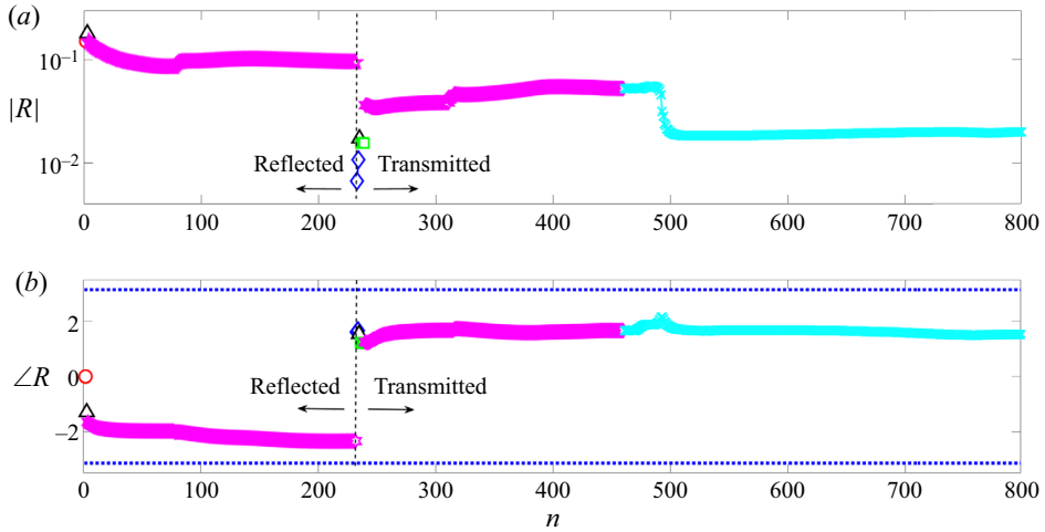
Figure 10. Evolution of the amplitude and phase of the reflection coefficient computed using the F-T model as a function of the number of modes considered. Markers and colours are the same as those used in figures 4 and 6 to identify the mode families. (a) amplitude, (b) phase. Blue dotted lines indicate \pm\pi in the phase plot.
