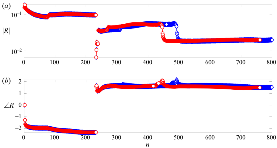
Figure 18. Evolution of the reflection coefficient as a function of the number of modes considered using the F-T model: blue \diamond refer to results obtained including near-sonic, downstream-travelling acoustic modes, red \circ refer to results obtained artificially removing near-sonic acoustic modes ( k_{aMAX}^+ = 3.2 ). (a) Amplitude, (b) phase.
